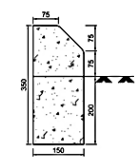
DETAIL OF KERB (Scale:- 1:10)
